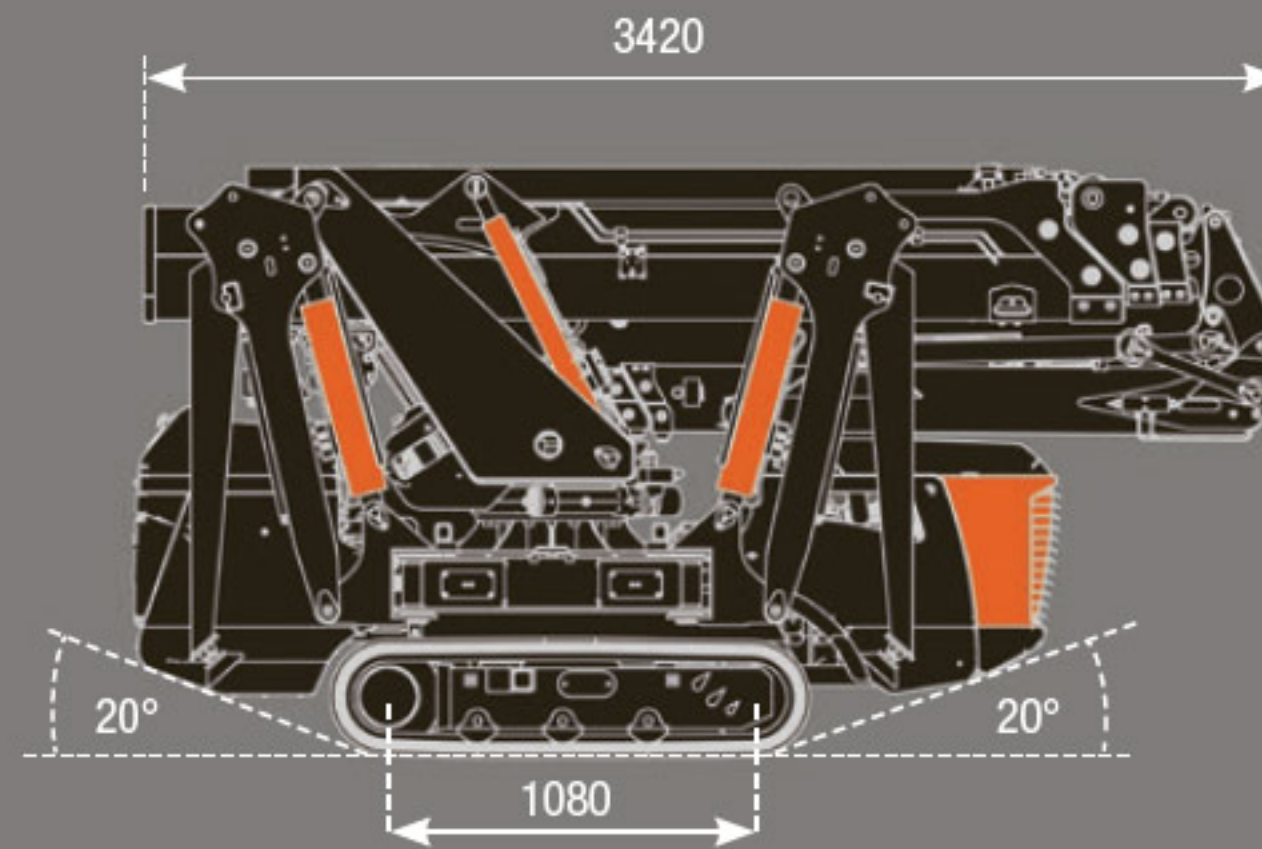
M 250 + Jib
